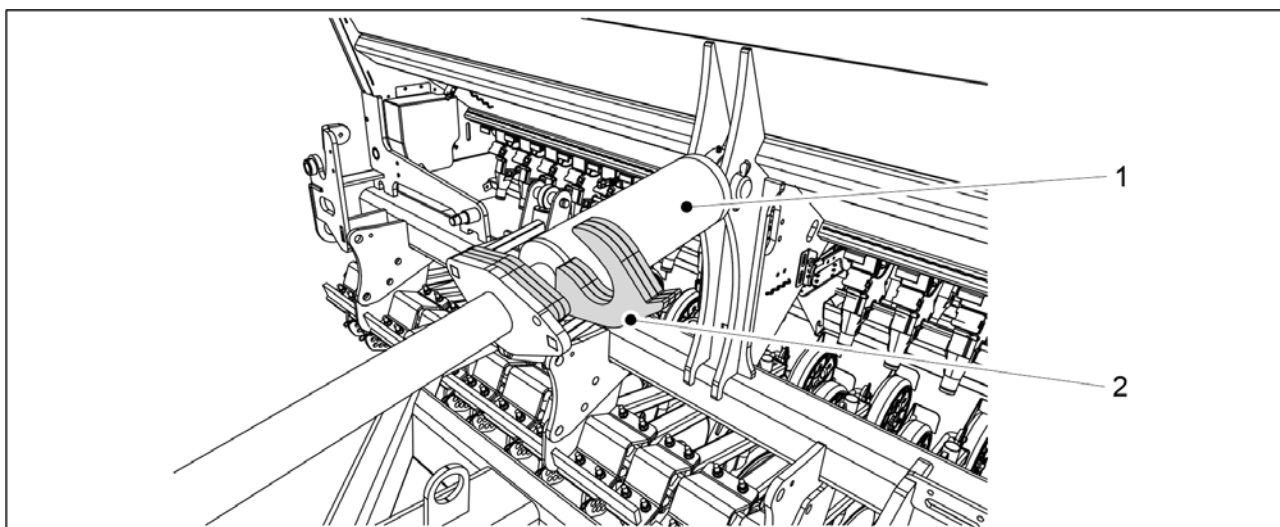
Bild. 5.3.4 - 122. Cylinderns justeringslameller
