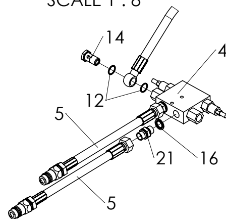
DETAIL A SCALE 1 : 8
